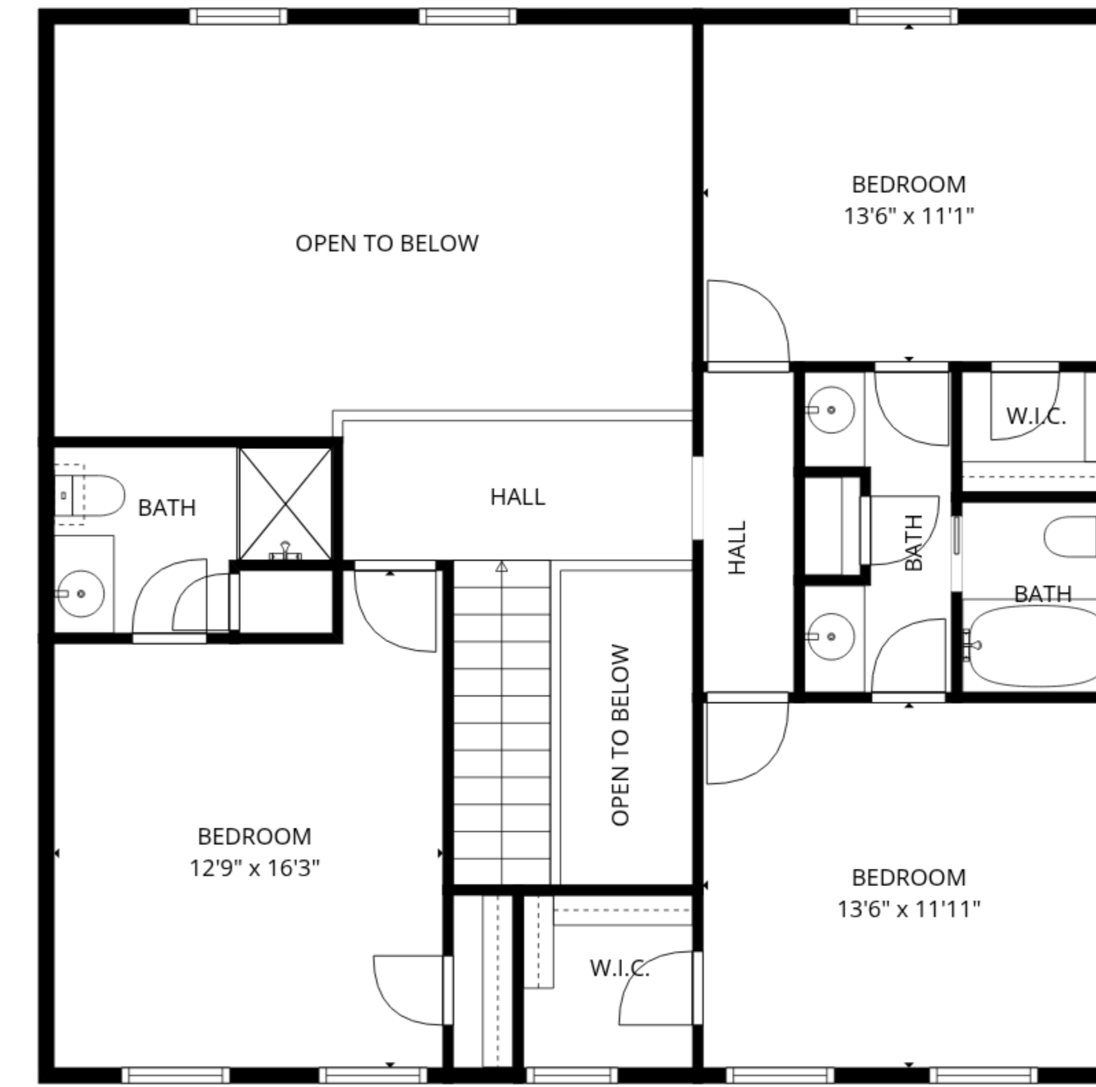
2nd floor
